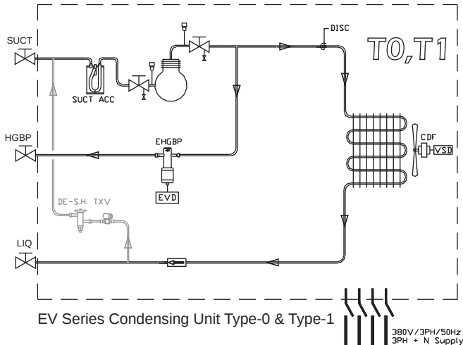
Refrigerant Diagram
